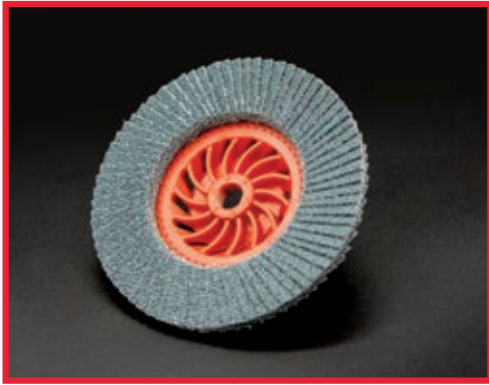
Vents in the plate for air circulation and additional material cooling.
